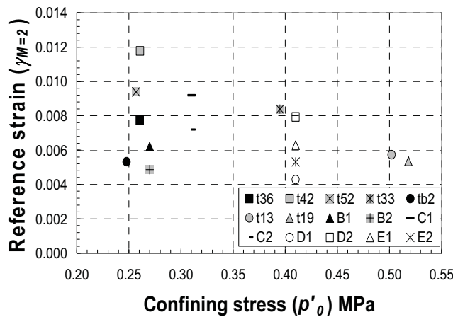
Fig. 7 Reference strain ( \gamma_{M=2} ) versus confining stress ( p'_0 ).
