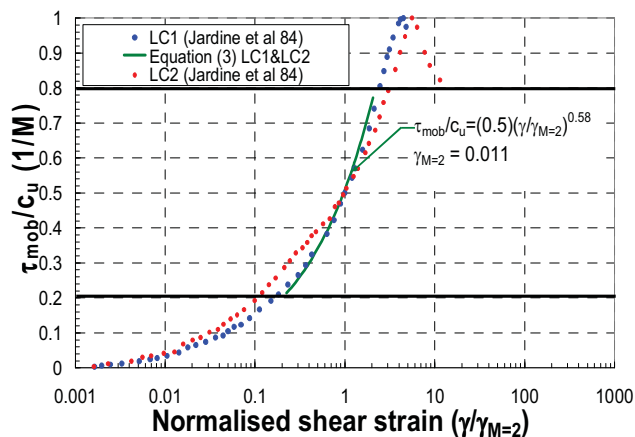
Fig. 5 Comparison of London clay data from Jardine et al (1984) with equation (3).
