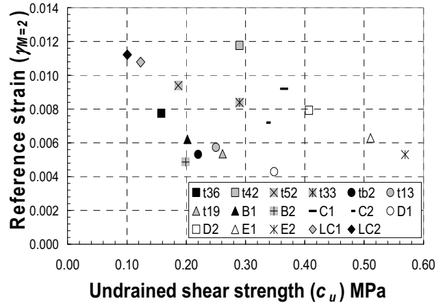
Fig. 9 Reference strain ( \gamma_{M=2} ) versus undrained shear strength ( c_u ).
