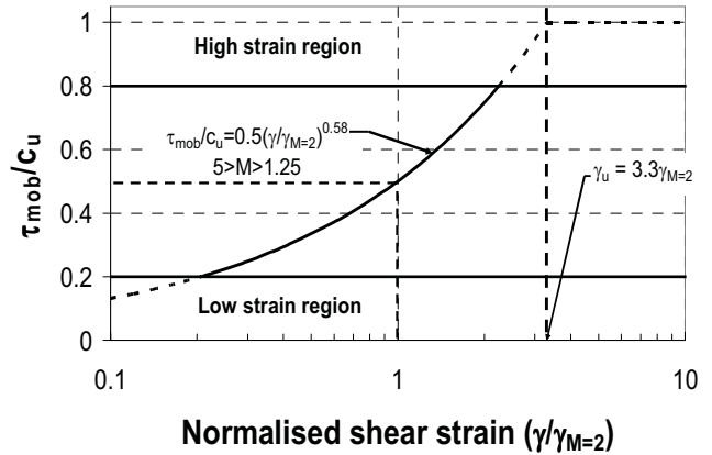
Fig. 3 Design stress strain for London clay.
