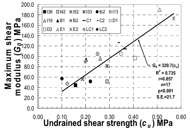
Fig. 10 Maximum shear modulus ( G_0 ) versus undrained shear strength ( c_u ) (London clay data)
