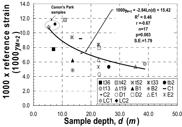
Fig. 6 Reference strain ( \gamma_{M=2} ) versus sample depth ( d ).
