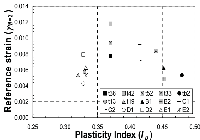
Fig. 8 Reference strain ( \gamma_{M=2} ) versus plasticity index ( I_p ).
