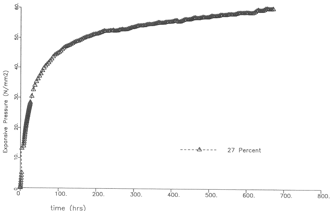
Figure 5 Expansive pressure versus time (Bristar 100) with 27% water
