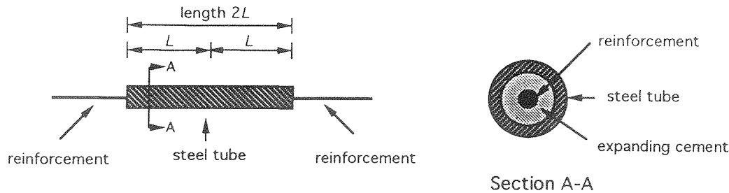
Figure 2 Coupling of reinforcement
