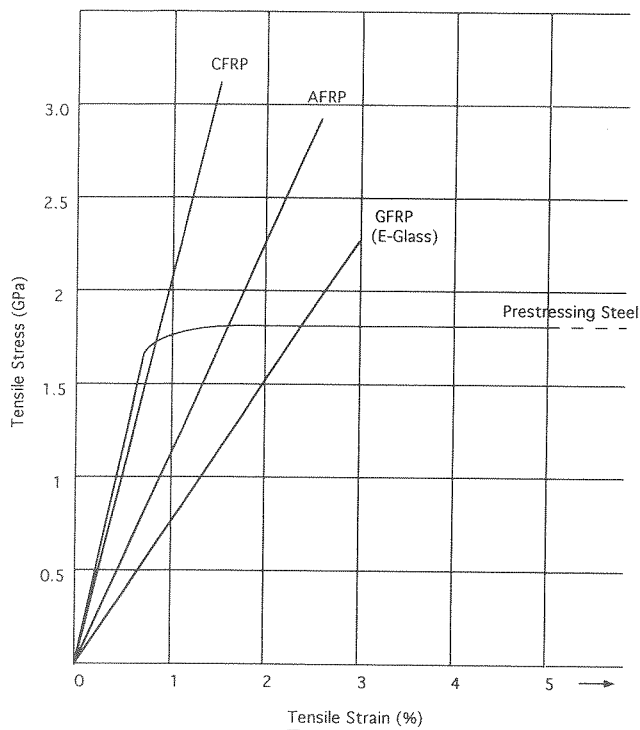
Figure 1 Stress-strain curves for different types of FRPs
