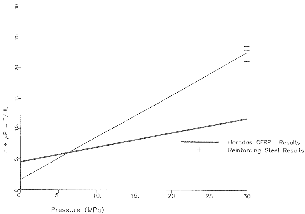
Figure 3 Graph of T/UL versus expansive pressure
