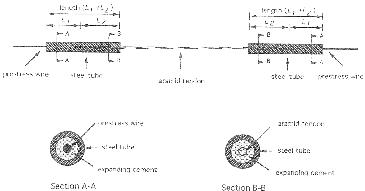
Figure 4 Steel/aramid/steel specimen
