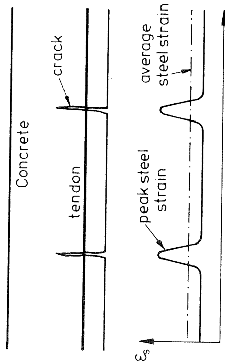
Figure 5. Actual strain distribution along tendon in a cracked beam.
