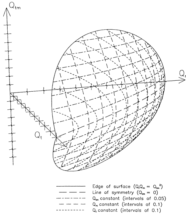
Fig. 2. Three-dimensional view of surface showing slope discontinuity.
