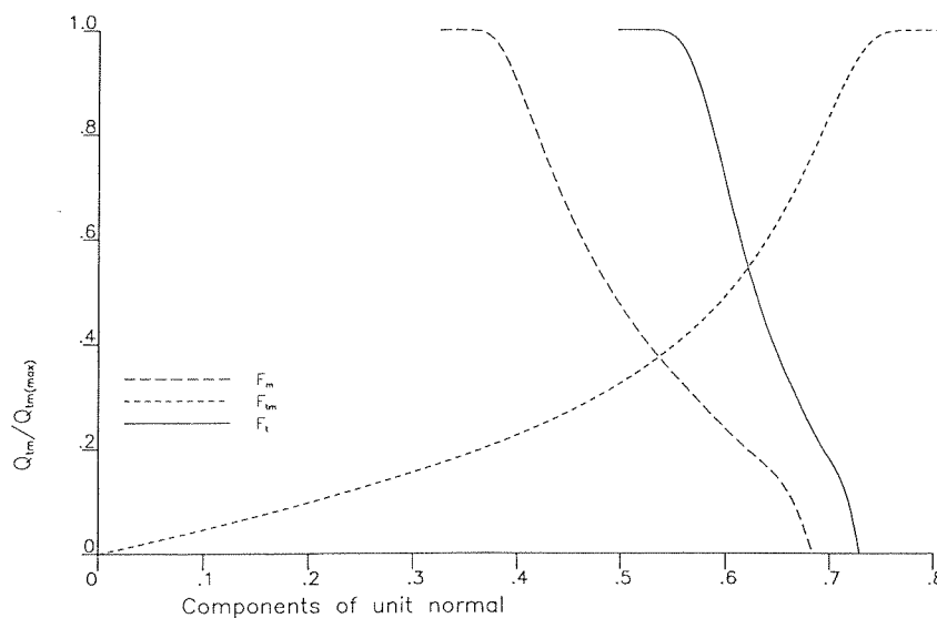
Fig. 9. Components of normal to yield surface along Q_t = Q_m .
