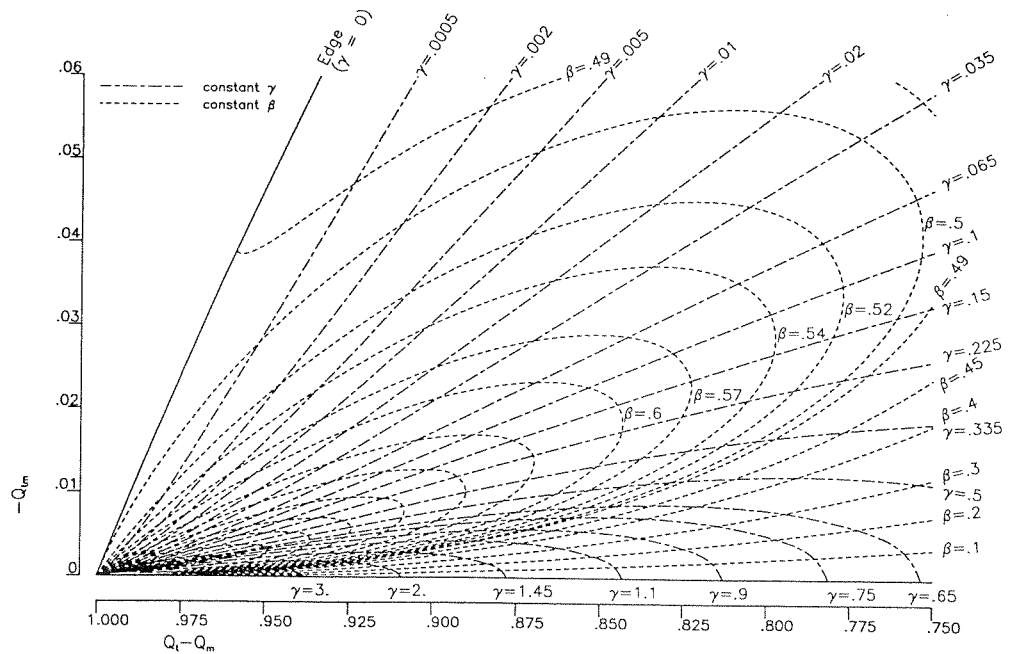
Fig. 8. Region corresponding to Ilyushin's in-plane dominant region. \beta, \gamma parametric plot.
