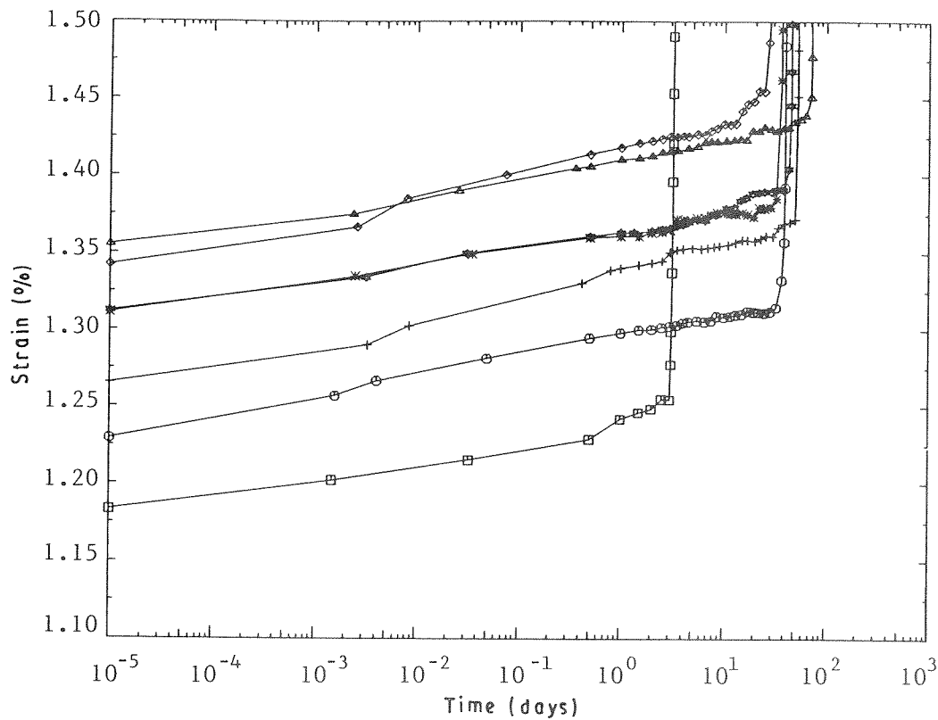
Figure 9 Strain versus logarithm of time (3 tonne ropes). ( \square ) C87-1, ( \circ ) C87-2, ( \triangle ) C87-3, ( \diamond ) C87-5, ( * ) C87-6, ( \times ) C87-7, ( + ) C87-8.
