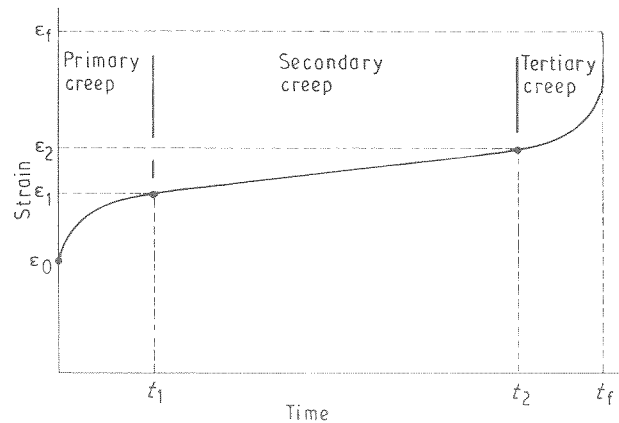
Figure 2 Creep curve.
