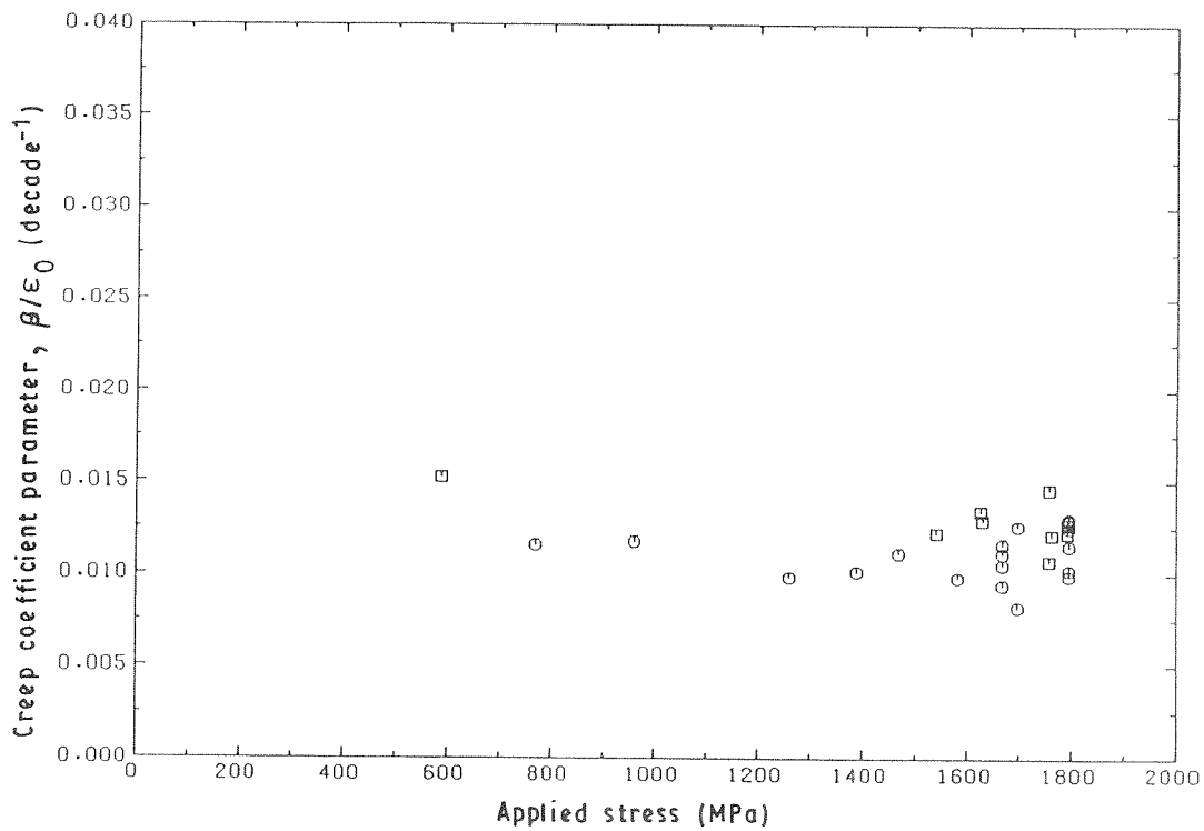
Figure 15 Stress dependence of the creep coefficient parameter, for ( \Delta ) 1.5 tonne and ( \odot ) 3 tonne ropes.
