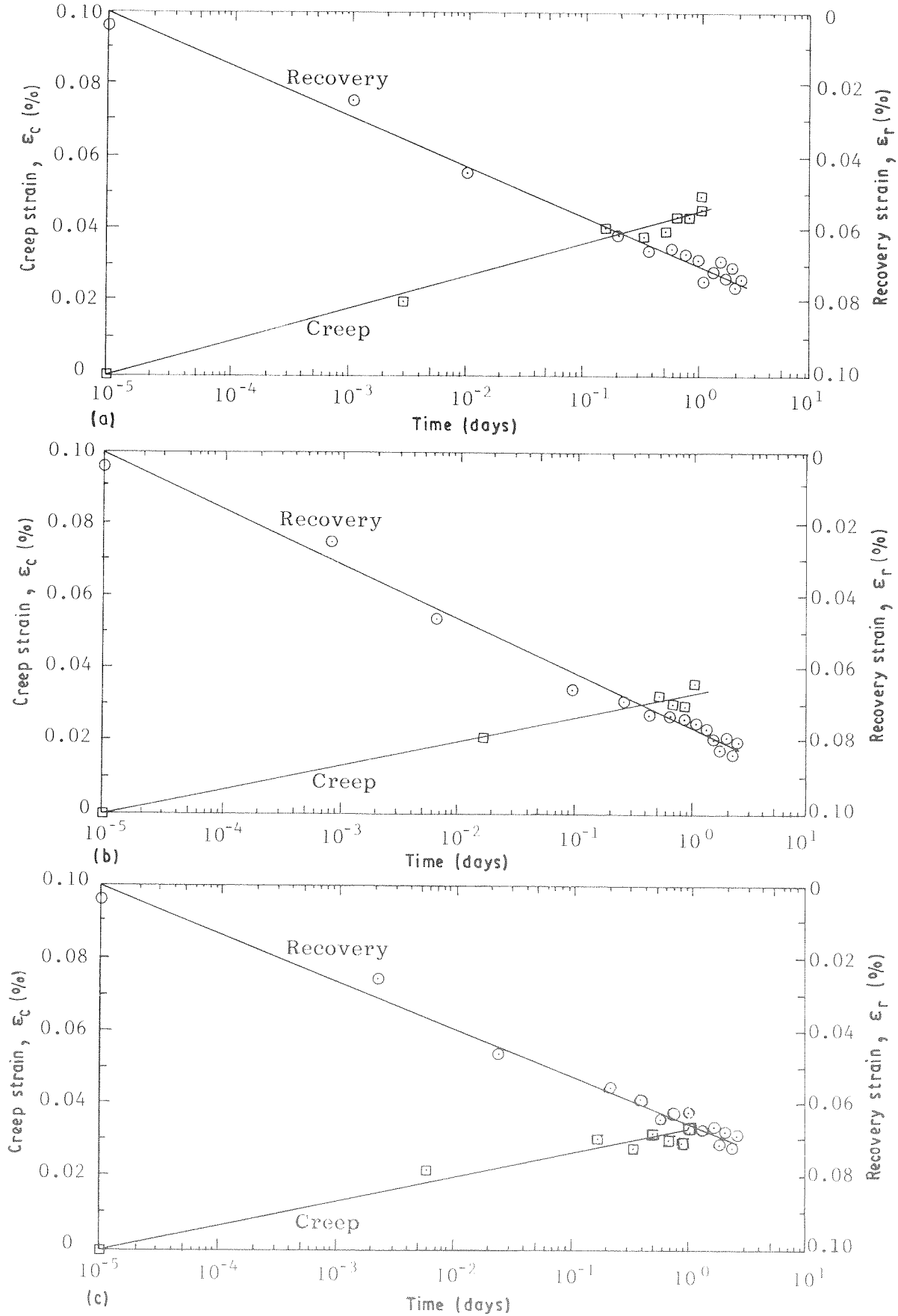
Figure 17 Creep and recovery at different stresses ( \epsilon_c and \epsilon_r as defined in Table V). (a) Specimen VR1, stress = 1368 MPa; (b) Specimen VR2, Stress = 1139 MPa; (c) Specimen VR3, stress = 913 MPa.
