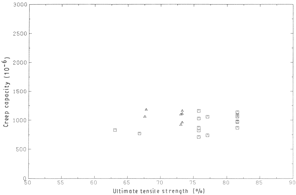
Figure 14 Creep capacity versus applied stress, for ( \Delta ) 1.5 tonne and ( \square ) 3 tonne ropes.
