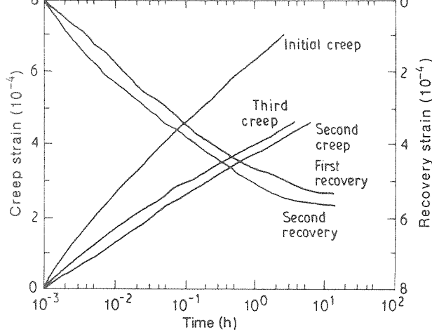
Figure 18 Repeated creep and recovery curves for Kevlar 49 filaments at room temperature. Creep load = 14.9 g [10].
