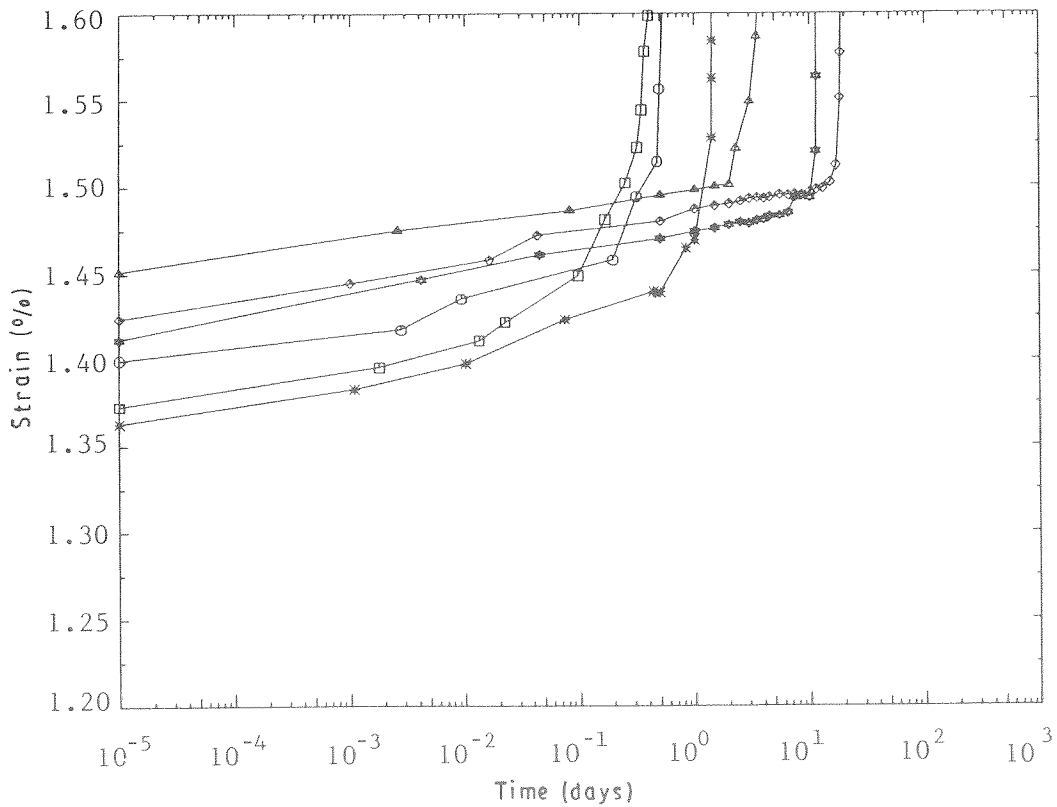
Figure 8 Strain versus logarithm of time (3 tonne ropes). (□) C93-1, (○) C93-2, (△) C93-5, (◇) C93-6, (*) C93-7, (☆) C93-8.
