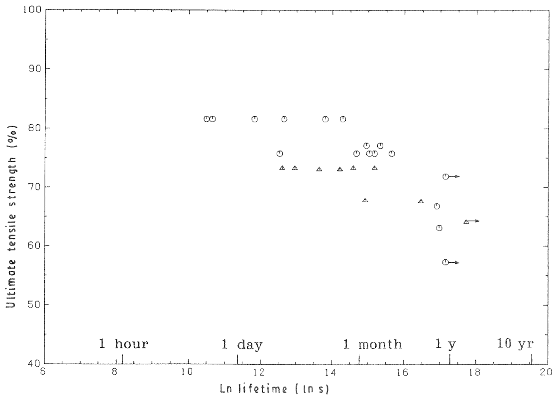
Figure 13 Applied stress versus lifetime, for ( \Delta ) 1.5 tonne and ( \circ ) 3 tonne ropes. ( \rightarrow ) Not failed.
