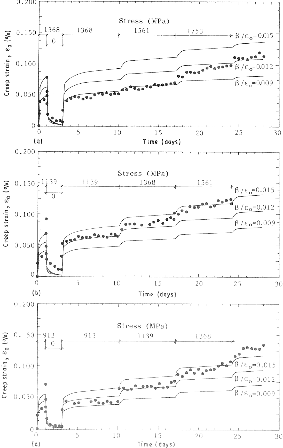
Figure 2f Comparison between (○) predicted and (●) observed creep strains of parallel-lay aramid ropes under varying loads, for (a) Specimen VR1, (b) Specimen VR2, (c) Specimen VR3.
