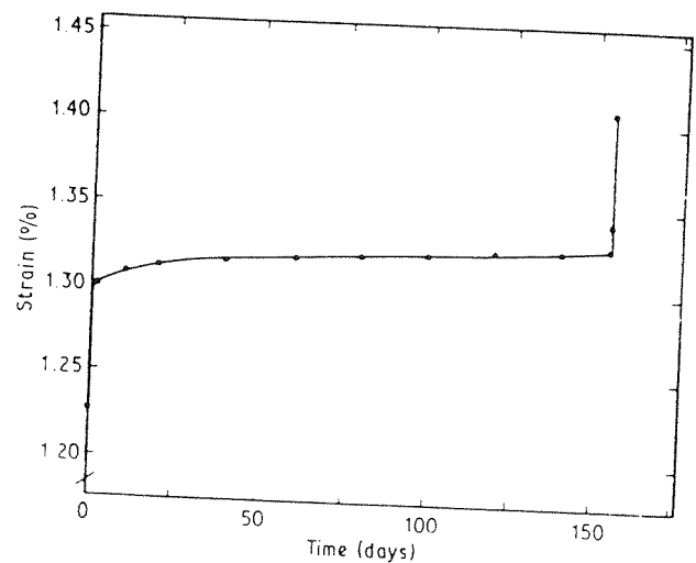
Figure 7 Creep strain curves for test 16.
