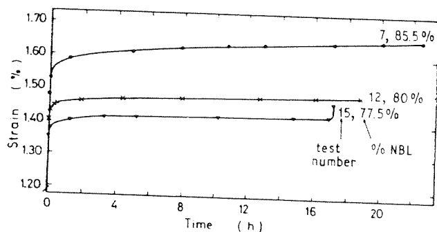
Figure 5 Creep strain curves for tests 7, 12 and 15.
