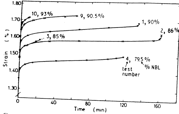
Figure 4 Creep strain curves for tests 1, 2, 3, 4, 9 and 10.
