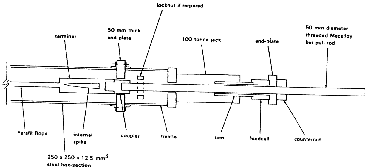
Figure 2 Laboratory stressing system for 60 tonne rope.
