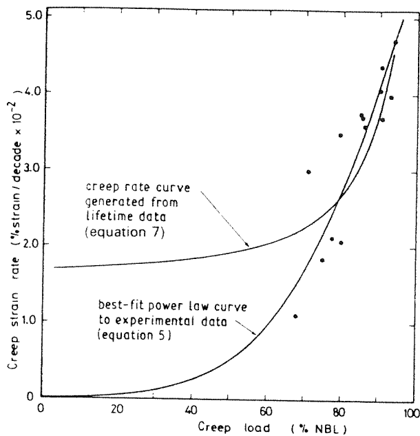
Figure 13 Creep strain rates plotted against load.
