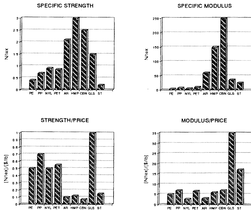
Fig. 1 Fibre property values: indicative only (all values cover a range for different types) PE=polyethylene; PP=polypropylene; NYL=nylon; PET=polyester; AR = aramid; HMP=high-modulus polyethylene; CBN=carbon; GLS=glass; ST=steel Unit of specific stress: N/tex = GPa/(g/cm^3) Unit of linear density: tex = g/km
